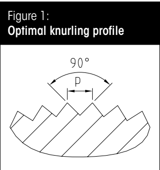
p = pitch
